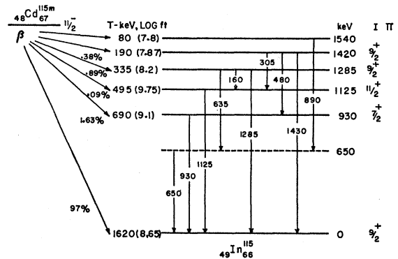
FIG. 1. Decay scheme of Cd^{115m} . The spin and parity assignment to the 930-, 1125-, 1285-, and 1420-keV levels are made from the present work.
